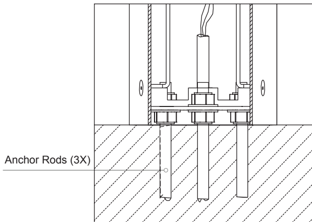
Mounting Details
